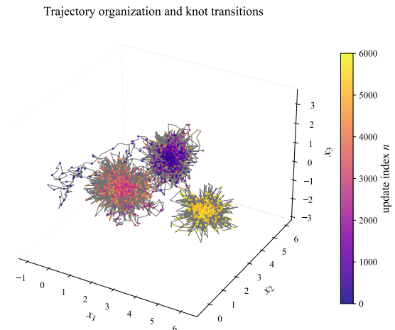
FIG. 3. Organization of a trajectory into multiple knot-like regions in state space. The continuous line shows the full trajectory, while discrete points indicate sampled positions contributing to the memory distribution. Color denotes the update index n . Shown is a representative run illustrating metastable clustering in one parameter regime.
