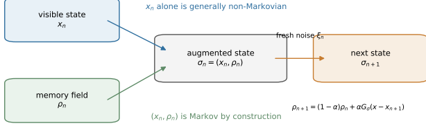
FIG. 1. Memory-state Markov embedding. The visible coordinate x_n is generally non-Markovian by itself, because the next update depends on the accumulated memory field \rho_n . Once \sigma_n = (x_n, \rho_n) is used as the state, all past influence enters through \rho_n , while fresh randomness enters through \xi_n .
