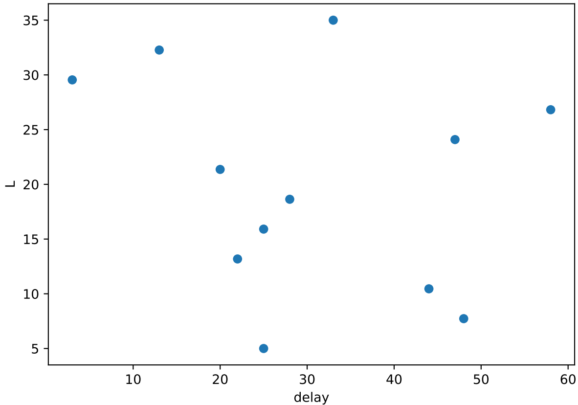
diffusive: Light Cone
