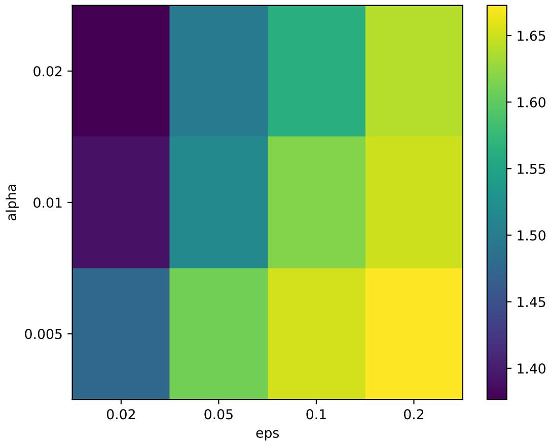
Fractal dimension Docc (mean over B, dim)
