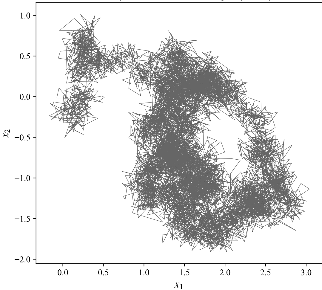
Memory-driven self-avoiding trajectory
