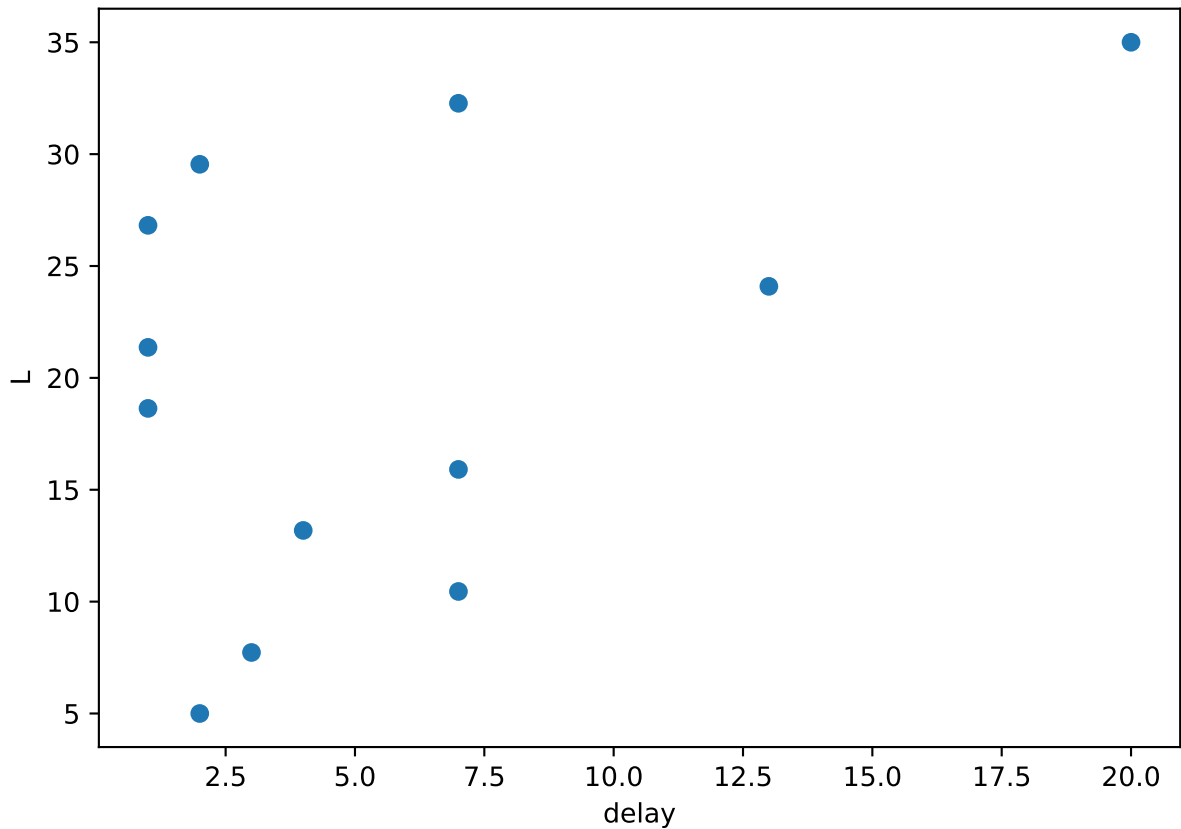
front: Light Cone
