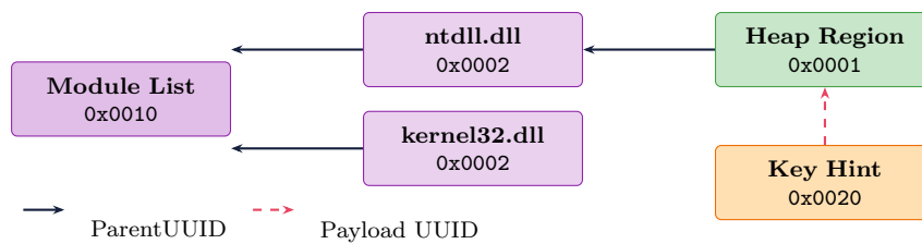
Figure 18: Block cross-referencing.
