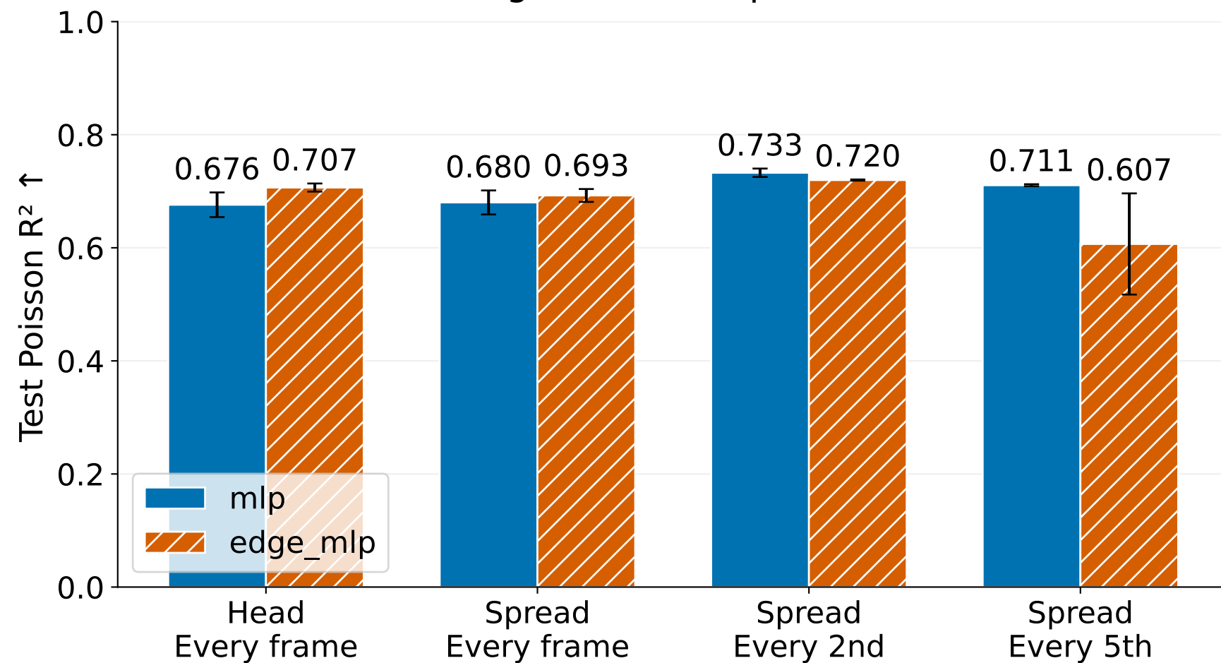
Observed through frame 15; predict to frame 115
