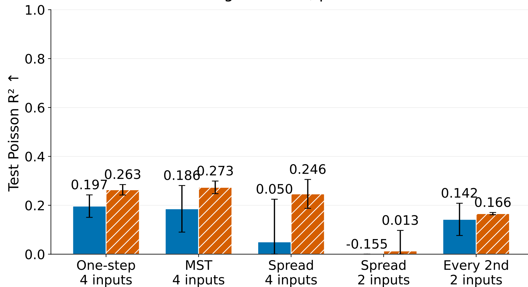
Observed through frame 3; predict to frame 103
