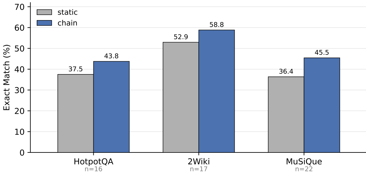
Exact Match under matched budget (qwen3.8-27b)
