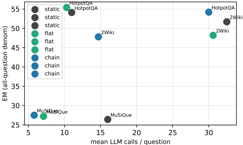
RQ2: cost frontier (LLM calls vs EM)
