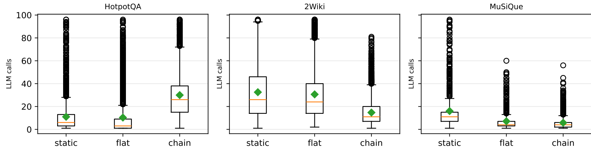
LLM-call distribution by arm (answered questions)
