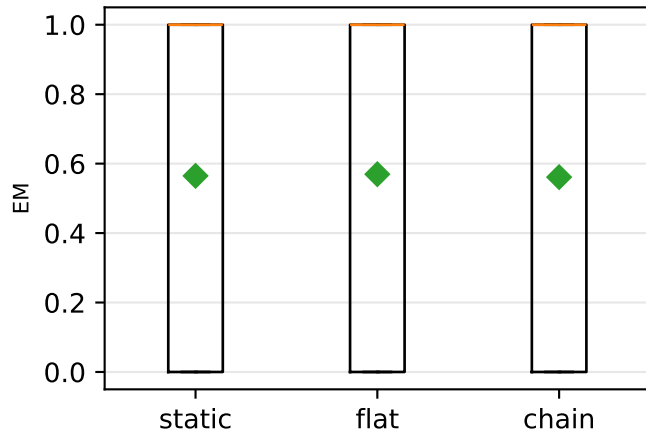
HotpotQA
