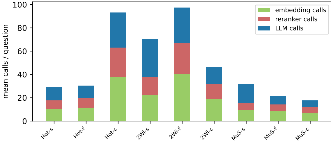
Invocation composition by arm
