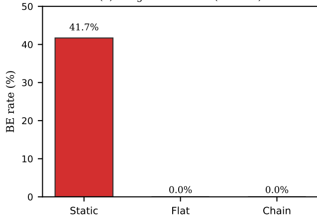
(b) Budget exhaustion (n = 350)
