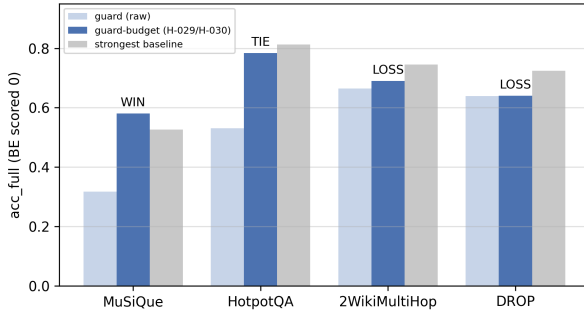
Figure 1: Matched-budget acc_full (budget-exceeded scored 0) for guard, guard-budget (H-029/H-030), and the strongest adapted baseline per dataset. Verdict per the 0.03 WIN/TIE/LOSS threshold. Strongest-Baseline Coverage is 1 out of 4 = 25 percent.
