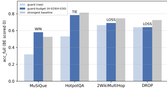
Figure 1: Matched-budget \text{acc}_{\text{full}} (budget-exceeded scored 0) for guard, guard-budget (H-029/H-030), and the strongest adapted baseline per dataset. Verdict per the 0.03 WIN/TIE/LOSS threshold. Strongest-Baseline Coverage is 1 out of 4 = 25 percent.
