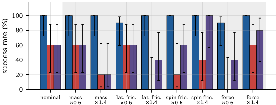
(a) success under execution-only mismatch (Wilson 95% CI)
