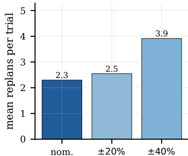
(b) PushAround replanning effort
