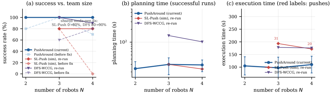
Figure 4: Robot-team scaling after the shared mode-generation fix, with the pre-fix runs shown as dashed history. (a) Success rate: the refinement lifts N=4 from 70% to 100% for PushAround, from 0% to 80% for SL-Push (sim) and from 80% to 90% for DFS-WCCG. (b) Planning time and (c) execution time of successful runs; the annotations in (c) are the push counts of SL-Push (sim), which needs twice as many pushes as PushAround.
