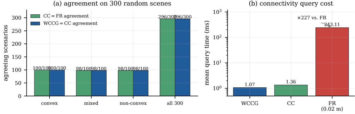
Figure 5: WCCG validation. (a) Agreement per category: CC and FR differ on 4 of 300 scenes (all raster-unstable), whereas WCCG matches the continuous reference on all 300 with zero false positives/negatives. (b) Mean connectivity-query cost on a logarithmic scale.
