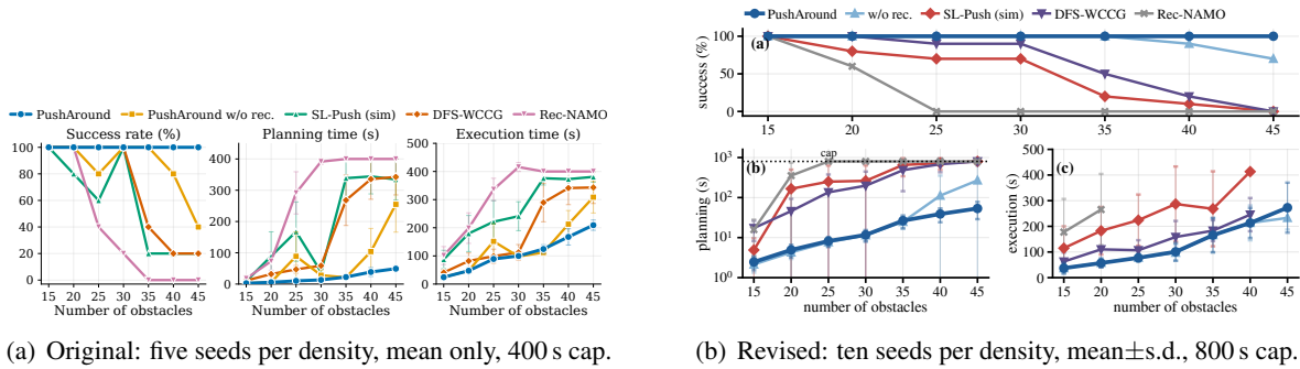
Figure 7: Obstacle-density scaling, original (left) versus revised (right). The panel structure is unchanged, so the two images are directly comparable: the revision doubles the number of independent seeds per density, adds one-standard-deviation error bars to both timing panels, and caps unsuccessful trials at the 800 s budget instead of 400 s, so failed runs are no longer displayed as favourable planning times.
