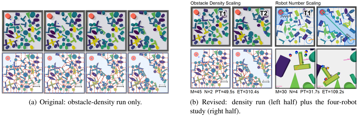
Figure 9: Simulation scenes of the scalability evaluation, original (left) versus revised (right). The revised figure covers both scalability axes instead of the obstacle-density axis alone: its left half keeps the representative M=45 , two-robot run (snapshots above, WCCG overlays with the start face in blue below), while its right half adds the four-robot study ( M=30 , N=4 ) with the global initial and final states above and two magnified views of a single pushing task below. This supplies visual evidence for the team-size results of Table III (Page 7), which previously had no accompanying figure.
