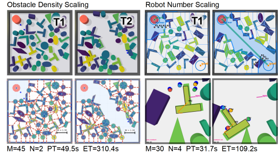
Fig. 9. Scalability of the clearing process. Left : obstacle-density scaling ( M=45 objects, two robots): snapshots during the clearing (top) and WCCG overlays with the start face in blue (bottom). Right : robot-team scaling ( M=30 objects, four robots): initial and final states (top) and zoomed views of one push before contact and during execution (bottom).
