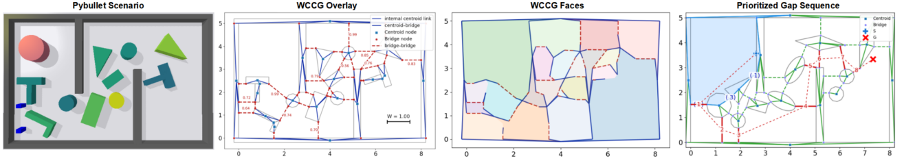
Fig. 3. Illustration of the W-clearance connectivity graph (WCCG) and gap ranking. From left to right: cluttered PyBullet scenario, WCCG overlay with centroid nodes, bridge nodes, and annotated gap widths, induced WCCG faces, and the prioritized frontier-gap sequence.
