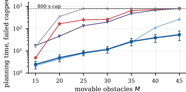
(b) planning time (10 seeds, mean \pm s.d.)
