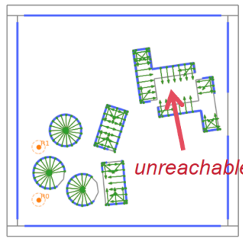
Robot Reachset
