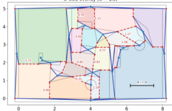
Sim-in-the-loop Search
