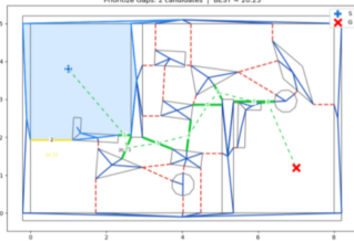
Gap Ranking
