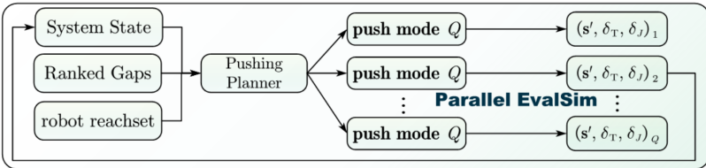
Sim-in-the-loop Search
