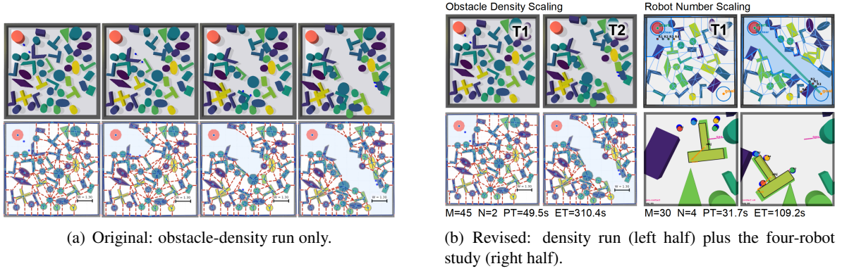
Figure 10: Simulation scenes of the scalability evaluation, original (left) versus revised (right). The revised figure covers both scalability axes instead of the obstacle-density axis alone: its left half keeps the representative M=45 , two-robot run (snapshots above, WCCG overlays with the start face in blue below), while its right half adds the four-robot study ( M=30 , N=4 ) with the global initial and final states above and two magnified views of a single pushing task below. This provides a qualitative illustration of the team-size results in Table III (Page 7), which previously had no accompanying scene figure.
