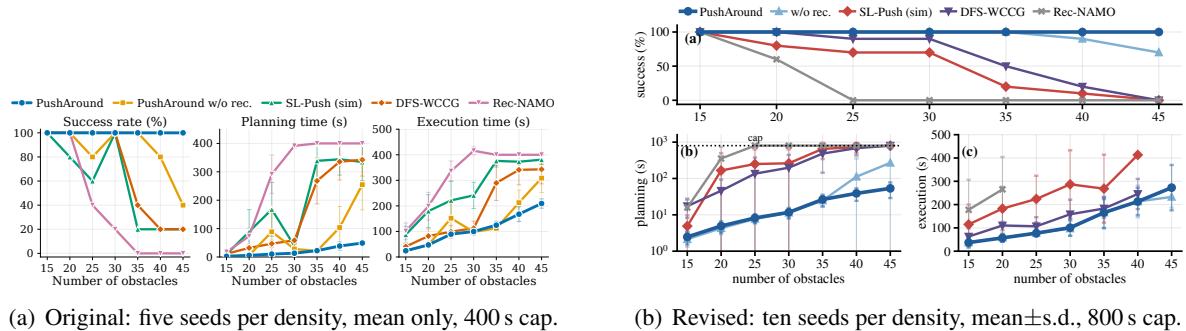
Figure 8: Obstacle-density scaling, original (left) versus revised (right). The panel structure is unchanged, so the two images are directly comparable. The revision doubles the number of independent seeds per density, adds dispersion to the timing results, and aligns the failed-trial statistic with the actual 800 s per-trial timeout; the earlier manuscript used a 400 s cap in this summary.
