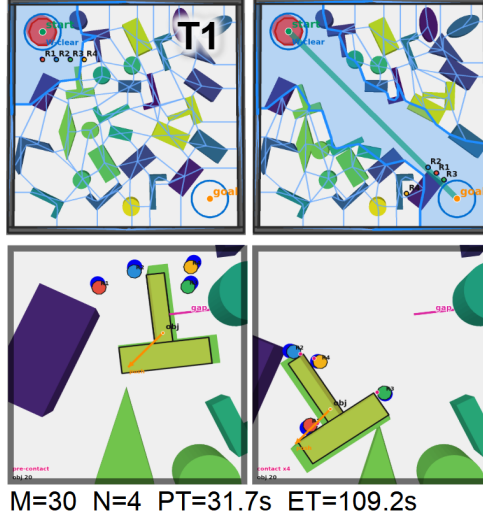
Figure 5: The four-robot study of the same evaluation ( M=30 , N=4 ): global initial and final states above, and two magnified views of a single pushing task (before contact and during the push) below.
