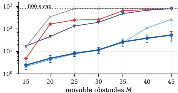
(b) planning time (10 seeds, mean±s.d.)
