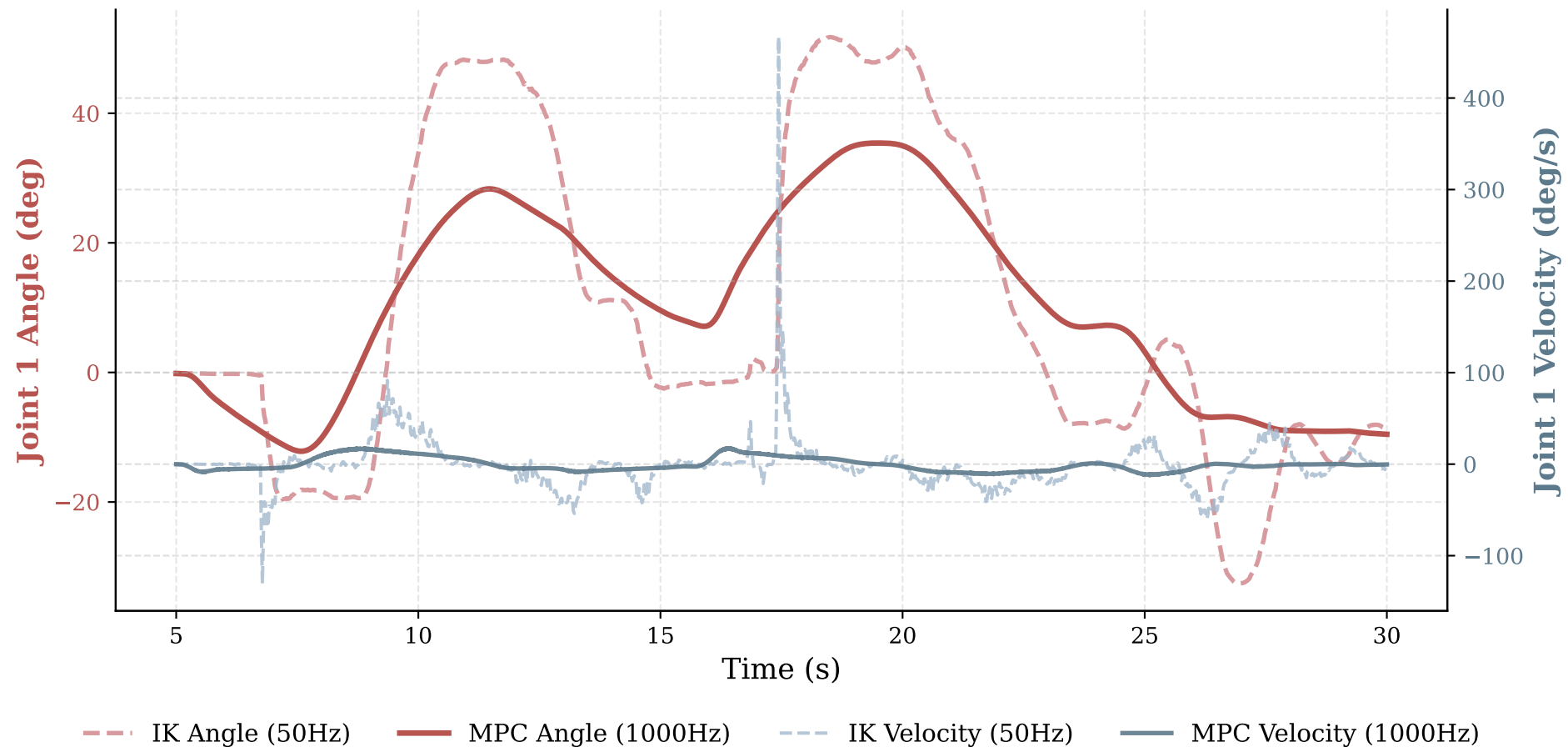
Tracking & Interpolation: Joint 1 (rokae_7dof)
