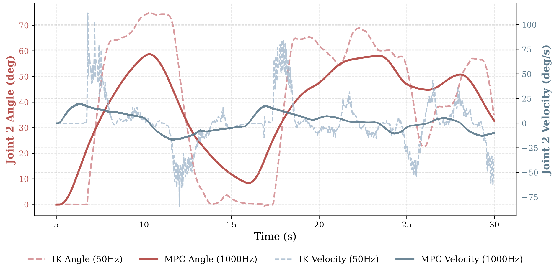
Tracking & Interpolation: Joint 2 (rokae_7dof)
