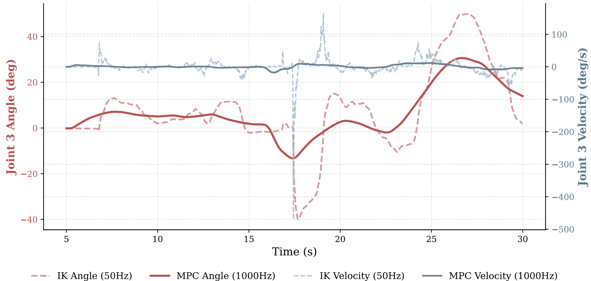
Tracking & Interpolation: Joint 3 (rokae_7dof)
