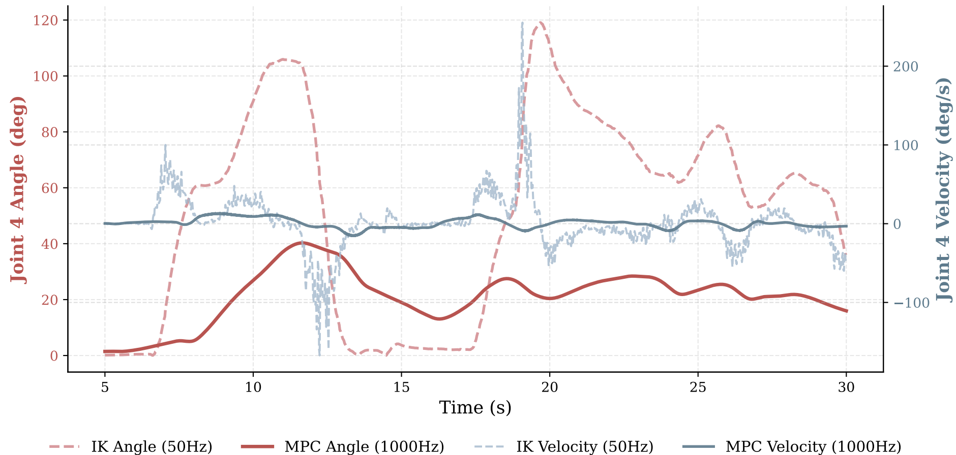
Tracking & Interpolation: Joint 4 (rokae_7dof)
