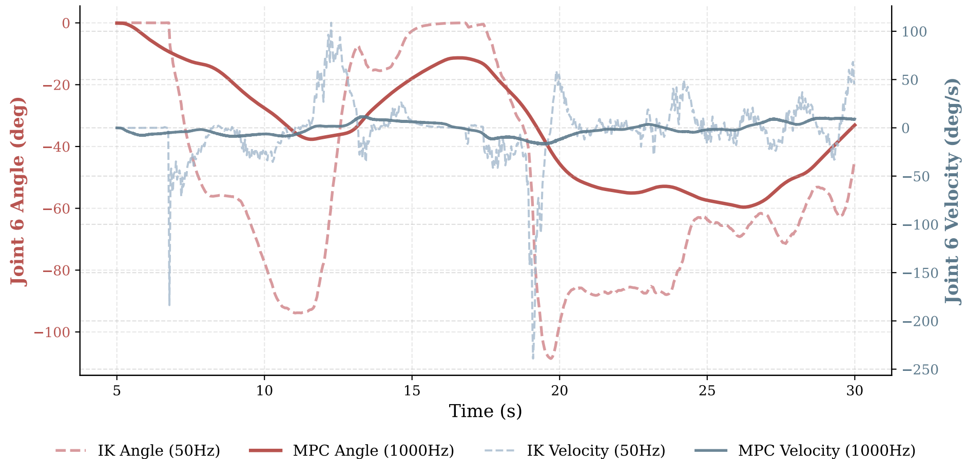
Tracking & Interpolation: Joint 6 (rokae_7dof)
