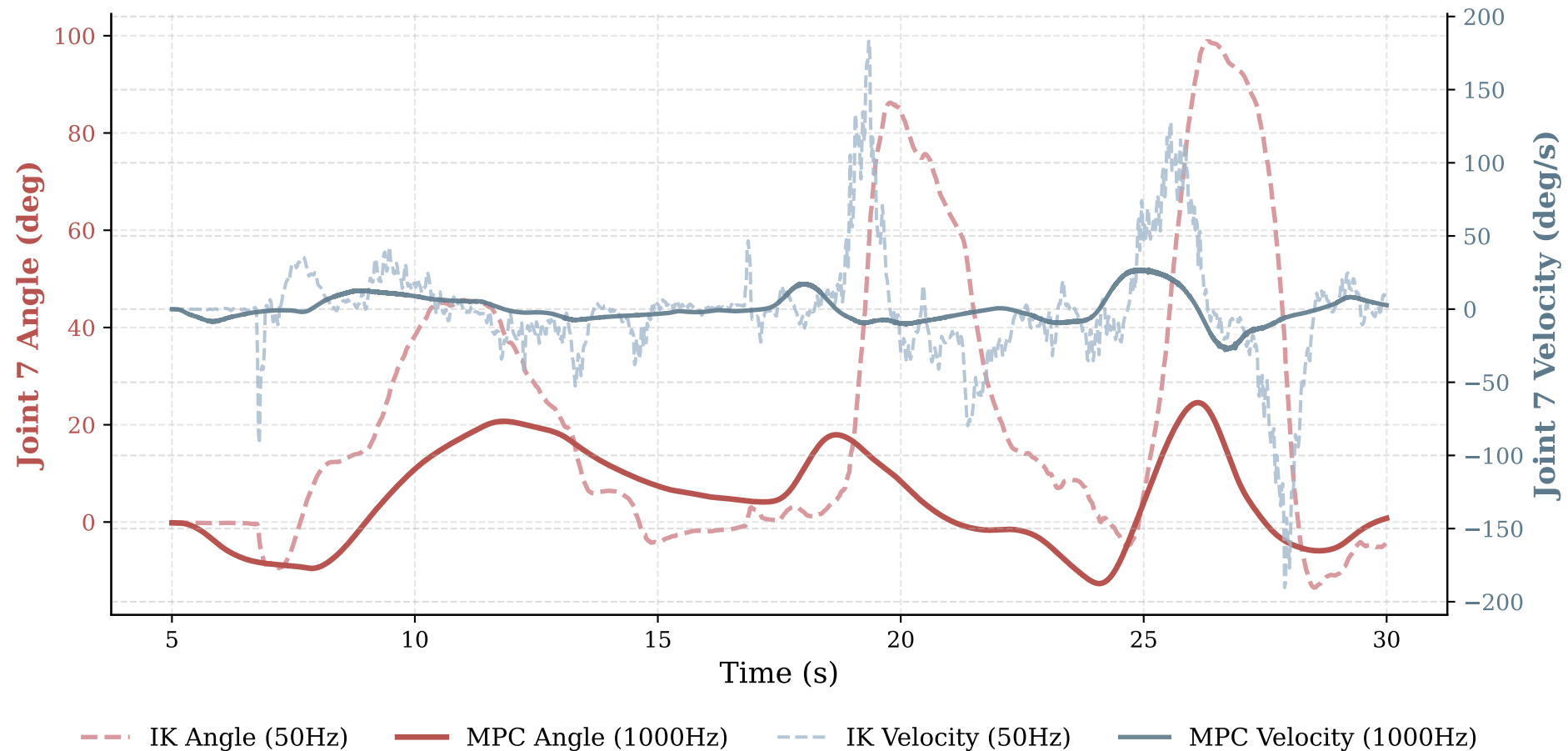
Tracking & Interpolation: Joint 7 (rokae_7dof)
