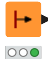
Image Reader
