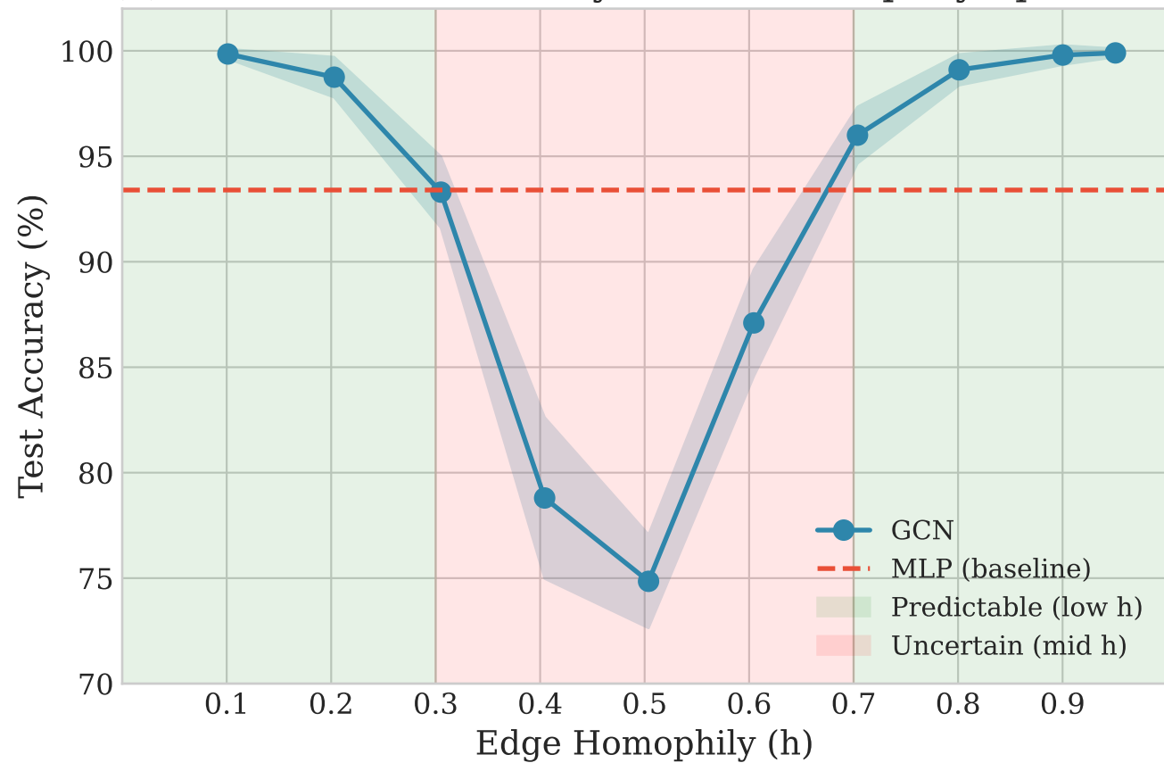
(a) GCN vs MLP Accuracy Across Homophily Spectrum
