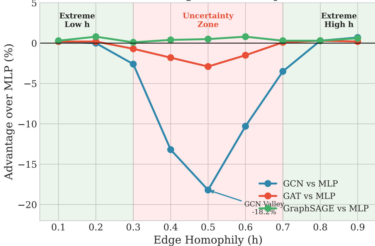
(b) GNN Advantage: The U-Shape Pattern
