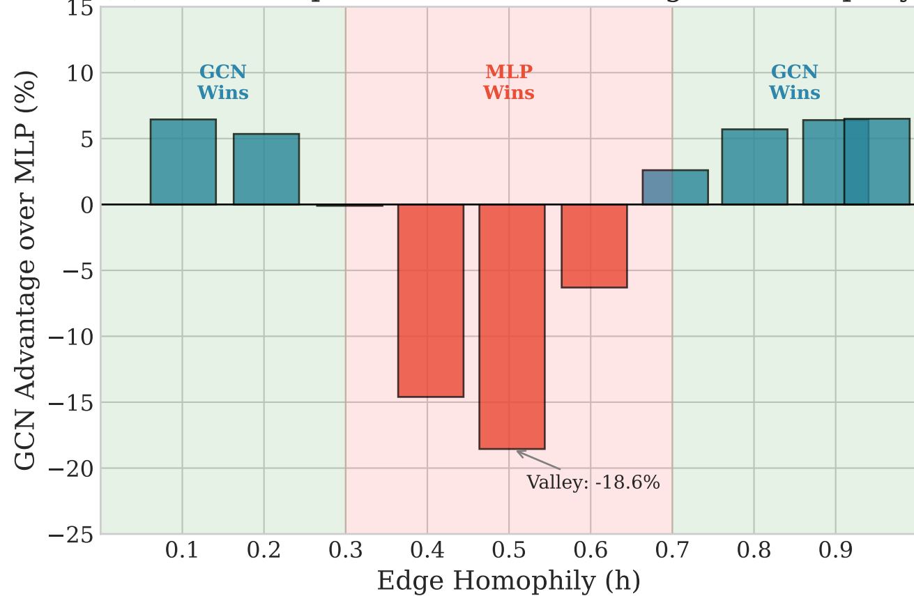
(b) The U-Shaped Law: GCN Advantage vs Homophily
