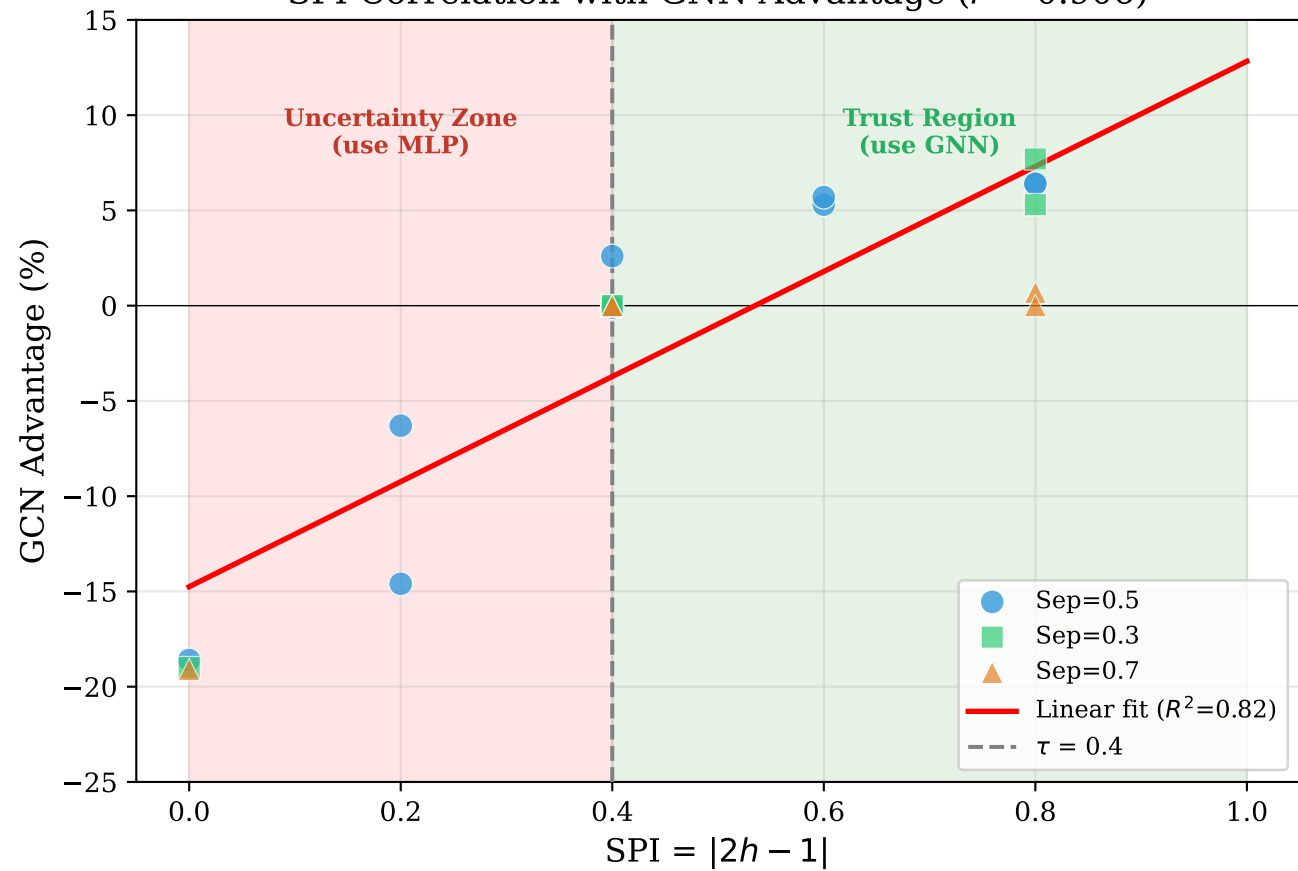
SPI Correlation with GNN Advantage ( r = 0.906 )
