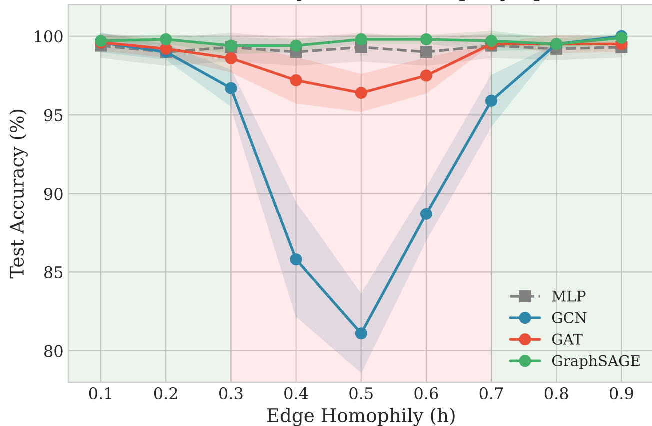
(a) Model Accuracy Across Homophily Spectrum
