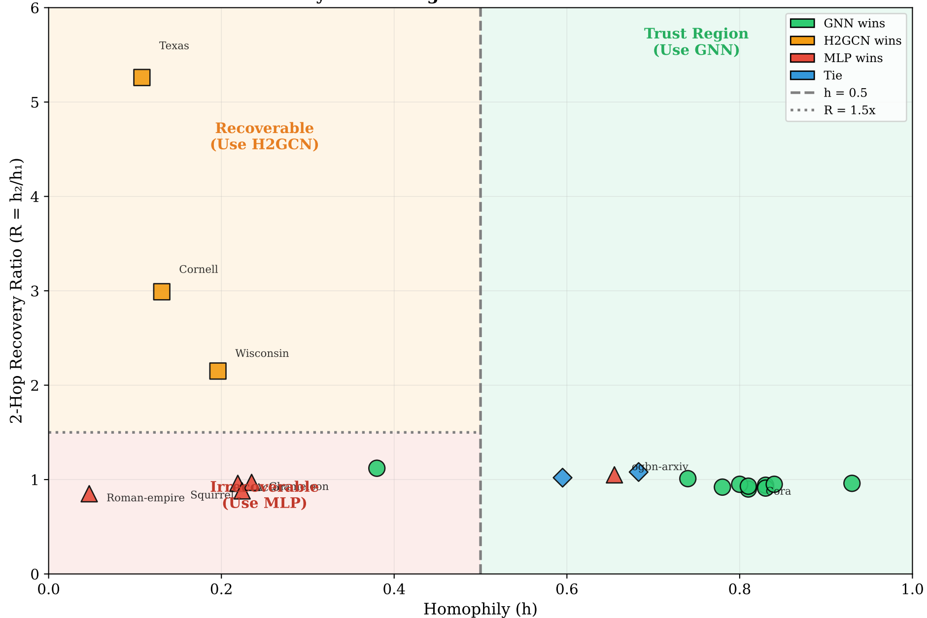
Decision Boundary Phase Diagram: Two-Factor Architecture Selection
