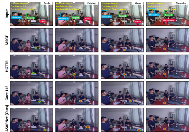
Fig. 4. Qualitative visual comparison among the attention prediction results obtained by different methods on the EASOAD.
