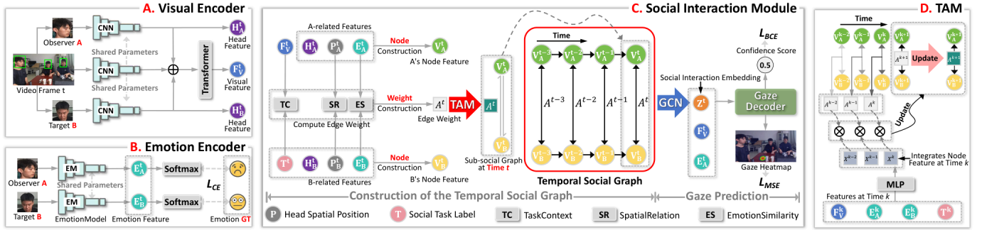
Fig. 3. Overview of EASAPNet. It is composed of four key modules: (A) a visual encoder for extracting scene and head features from video frames; (B) an emotion encoder for modeling the emotional states of the observer and the visible affective cues of the target; (C) a social interaction module, which builds a temporal social graph to capture dynamic social relations; and (D) a temporal attention mechanism (TAM) for adaptively aggregating temporal interaction information. The integration of these modules enables EASAPNet to jointly reason about visual cues, emotions, and social contexts for accurately predicting second-order attention.
