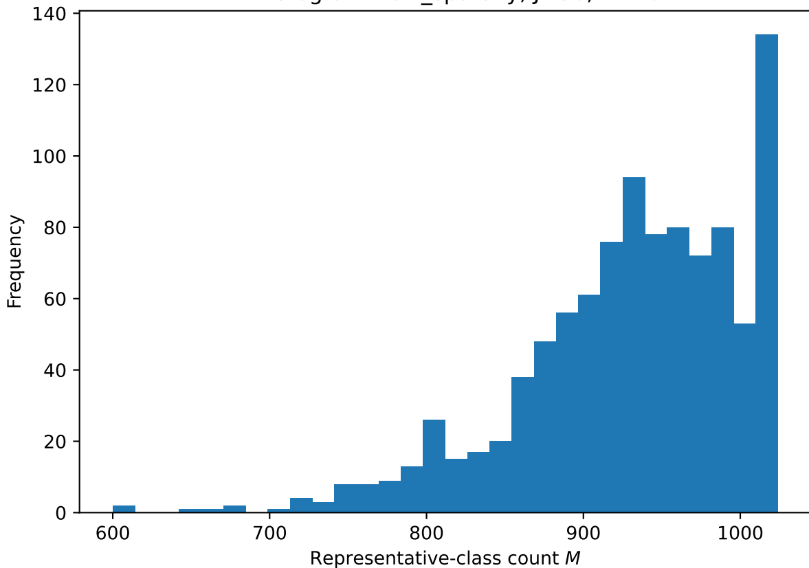
M histogram: row_sparsity, J=50, K=10
