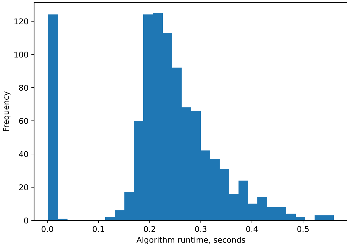
Runtime histogram: row_sparsity, J=50, K=10
