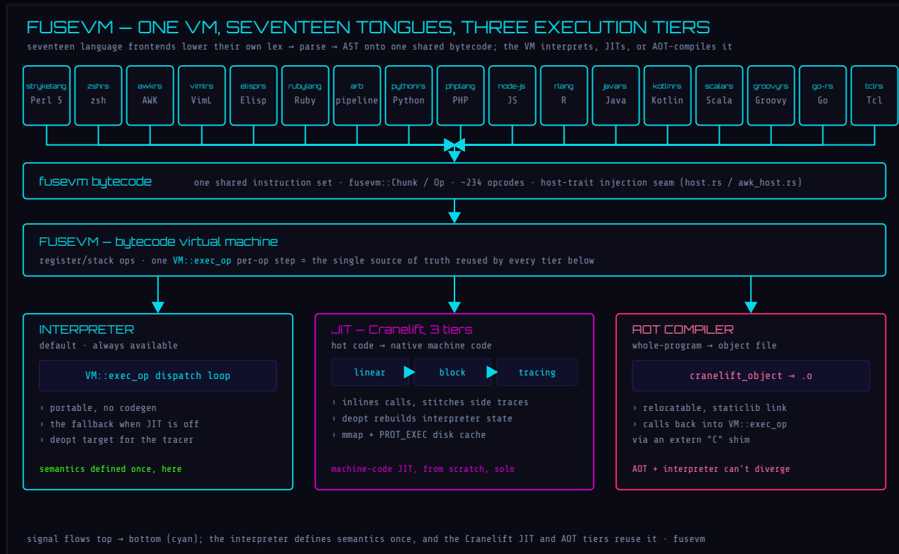
Figure 2: The fusevm execution engine: seventeen language frontends lower their own lex/parse/AST onto one shared bytecode, which the VM runs three ways — an interpreter (the semantic source of truth), a three-tier Cranelift machine-code JIT, and an AOT object compiler that both reuse the interpreter's per-op step.
