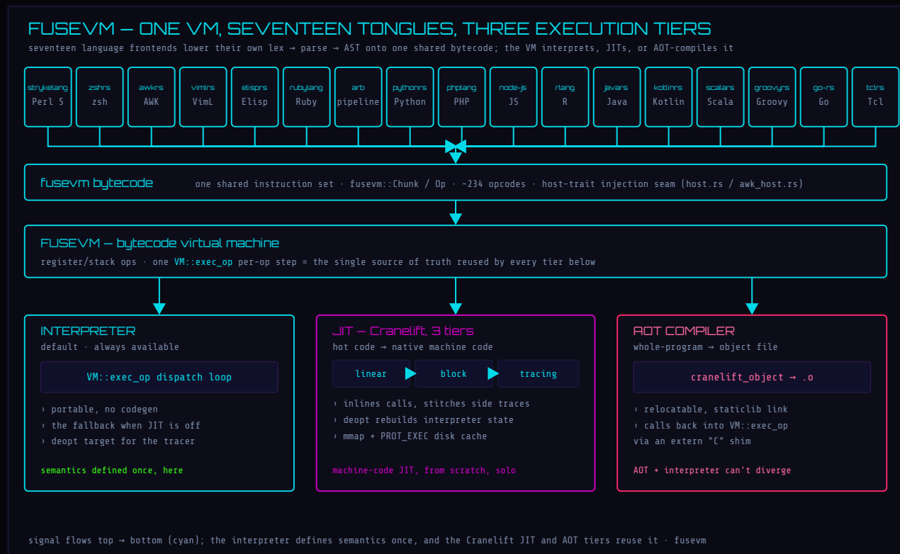
Figure 42: The fusevm execution engine: seventeen language frontends lower their own lex/parse/AST onto one shared bytecode, which the VM runs three ways — an interpreter, a three-tier Cranelift JIT, and an AOT object compiler — so every tool written once against the bytecode serves the whole family of tongues.
