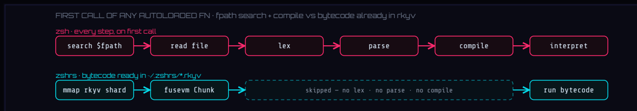
Figure 8: First call of any auto-loaded function – the majority of zsh's function surface: zsh searches $fpath then lex → parse → compile → interpret; zshrs mmmaps pre-compiled fusevm bytecode from the rkyv shard, skipping the entire compile pipeline.
