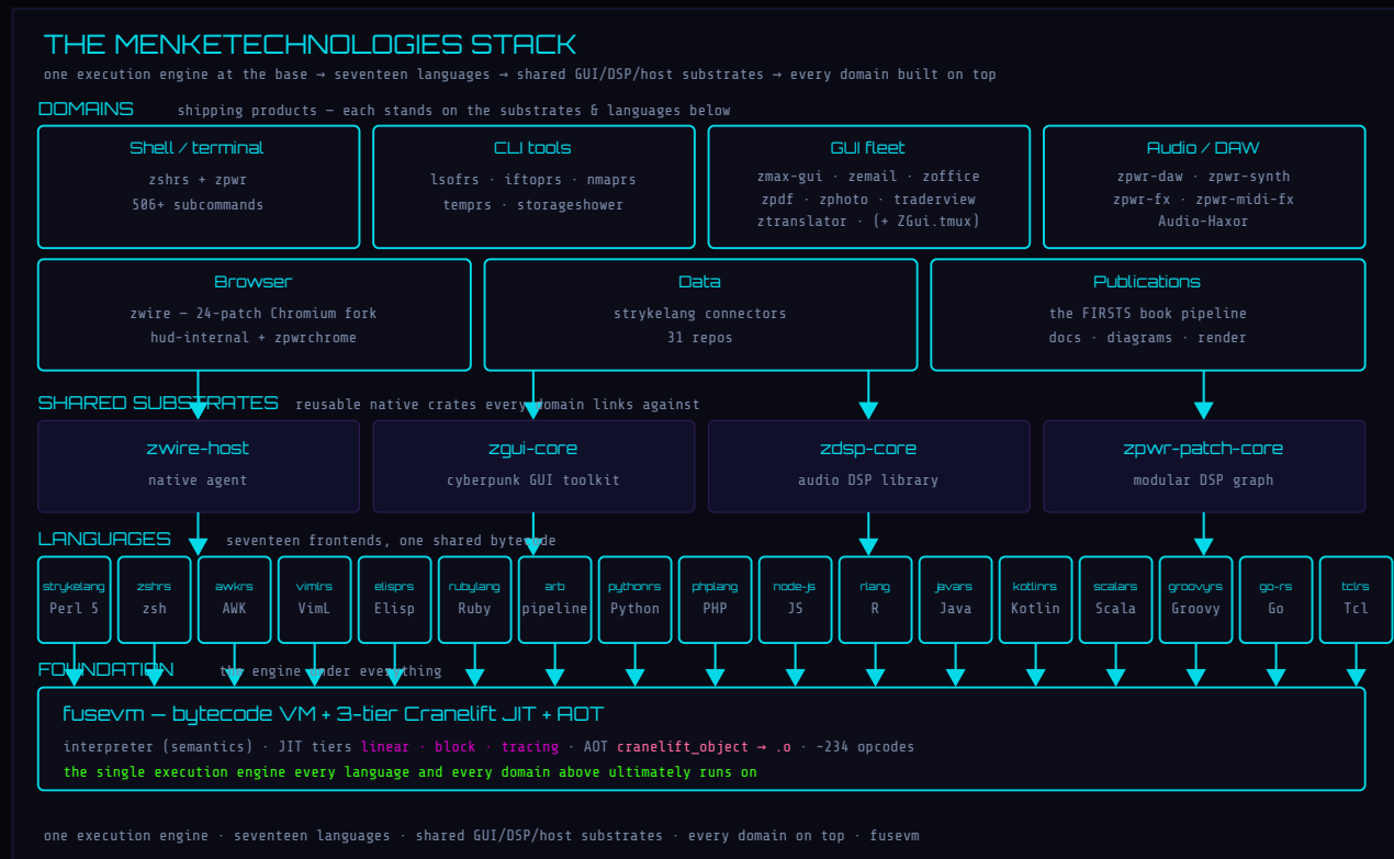
Figure 1: The whole stack at a glance: one execution engine (fusevm) under seventeen language frontends, a band of shared substrates (zwire-host, zgui-core, zdsp-core, zpw-patch-core), and the domains built on top — shell/terminal, CLI tools, the GUI fleet, audio/DAW, the browser, the data connectors, and this publications pipeline.
