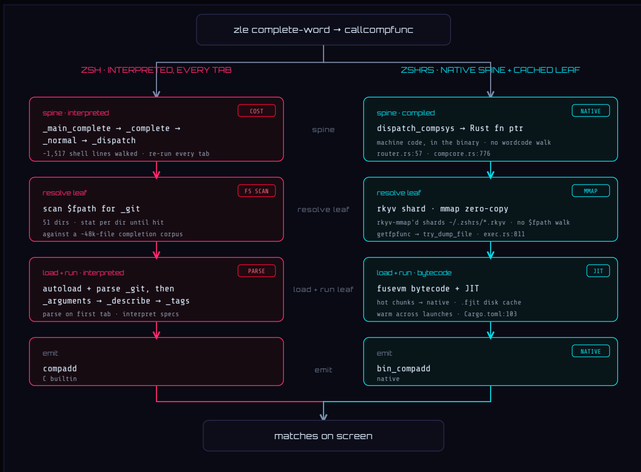
Figure 2: Tab completion, zsh vs zshrs: the interpreted spine and $fpath scan on every tab (left) versus a native Rust spine and an rkyv-mmap'd hash-index leaf resolve (right). The resolve-leaf step is an O(\text{fpath}) filesystem walk collapsed to an O(1) shard lookup.
