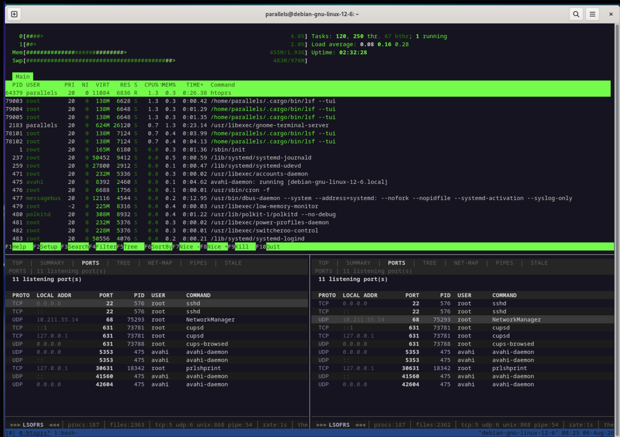
Figure 1: All three nouns in one terminal. The panes are the three framed regions, each an ordinary program that knows nothing about the multiplexer: htoprs across the top, and two lsfrs --tui clients below it. Together they are one window — one screenful, divided by a layout. The bar along the bottom is the status line, and it describes the session : [0] on the left is the session's name, then the session's window list, 0:htoprs* and 1:bash- , where * marks the window you are looking at and - marks the one you were on before. So the picture shows one of this session's two windows; pressing C-b 1 would replace everything above the bar with the other one, and the three programs here would keep running unattended. The right of the bar is the pane title, the clock, and the date. Nothing in the bar or the pane frames is a ztmux extension — no configuration file was loaded, so every field is the default in src/ported/options_table.rs , which Chapter 20 takes apart one at a time.
