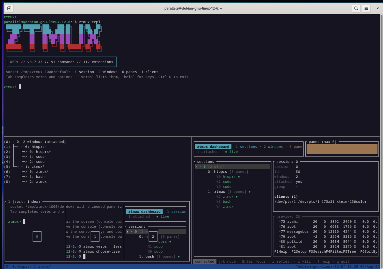
Figure 2: Three of the interactive surfaces at once. Top: ztmux repl ( src/extensions/repl.rs ), the standalone reedline console — banner with the live socket path and session/window/pane/client counts, then a prompt that runs every line exactly as ztmux <line> would, with Tab completing command names, aliases, extension verbs, and flags taken off each verb's args_parse template. Bottom left: choose-tree drawing the session/window/pane hierarchy through the ported mode_tree widget of Chapter 34. Bottom right: ztmux dashboard ( src/extensions/dashboard.rs ), the ratatui overview built on the same structured list-* -o json output any script can read. The console is not a wrapper around the client: it speaks to the same server over the same socket as every other entry point.
