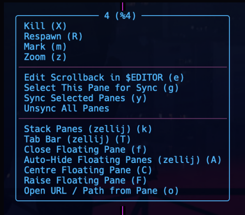
Figure 6: The default right-click pane menu, drawn by the ratatui layer's draw ( src/extensions/ratatui_ui.rs:309 ) from the same menu_data the ported path would draw: an item whose name is empty becomes a rule line, one whose name starts with - is rendered dimmed and unselectable — which is why Unsync All Panes carries no key here, its #{?synchronize-panes,, -} prefix having disabled it. The menu is defined once as format strings in src/ported/key_bindings.rs:52-90 , and the conditionals in those strings are what decide the contents: the splits and swaps are absent, and Close Floating Pane , Centre Floating Pane , and Raise Floating Pane are present, because every one of them tests #{?pane_floating_flag,...} and this click landed on a floating pane. The upstream items ( Kill , Respawn , Mark , Zoom ) sit above the ztmux ones (scrollback editing, the pane-sync marks, the zellij-mode toggles) in one list, because a menu is a list of command-language invocations and the extension entries are ordinary commands.
