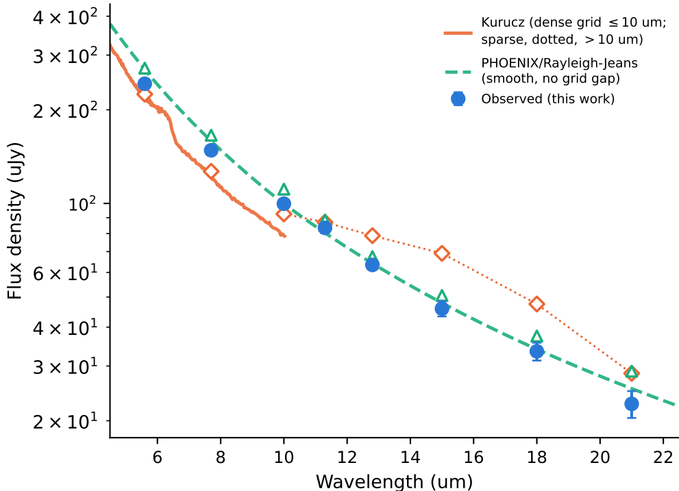
J1757132: observed vs. two independent model predictions
