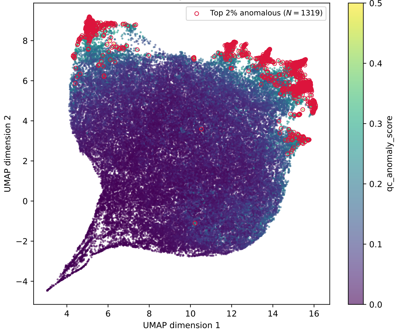
UMAP embedding of SED residuals
