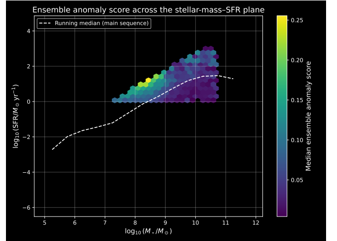
Figure 2. Stellar-mass–SFR plane for the full 64,195-source clean subsample with valid LePHARE mass/SFR fits, hexbinned and colored by the median ensemble anomaly score ( qc_anomaly_score ) per bin. The dashed white line is a running-median main-sequence trace (0.5 dex mass bins, \geq 10 sources/bin). Elevated scores concentrate above this trace rather than tracking its bulk (Mann-Whitney U test on ensemble score, above vs. at/below the main sequence, p < 10^{-300} ).
