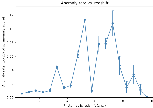
Figure 1. Flagged anomaly rate (top 2% of ensemble score among the 65,939-source clean sample) in \Delta z = 0.5 redshift bins from z = 0.5 to z = 10 . Error bars are Poisson uncertainties on the flagged count per bin. An OLS fit to the binned rate finds no significant redshift trend ( p = 0.32 ).
