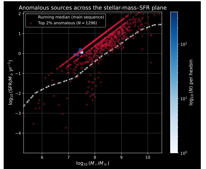
Figure 2. Top-2% flagged anomalies (crimson circles, N = 1,296 ) on the stellar-mass–SFR plane, against a hexbin density map of the full 64,195-source clean subsample with valid LePHARE mass/SFR fits. The dashed line is a running-median main-sequence trace (0.5 dex mass bins, \geq 10 sources/bin). Anomalies preferentially sit above this trace (Mann-Whitney U test on ensemble score, above vs. at/below the main sequence, p < 10^{-300} ).
