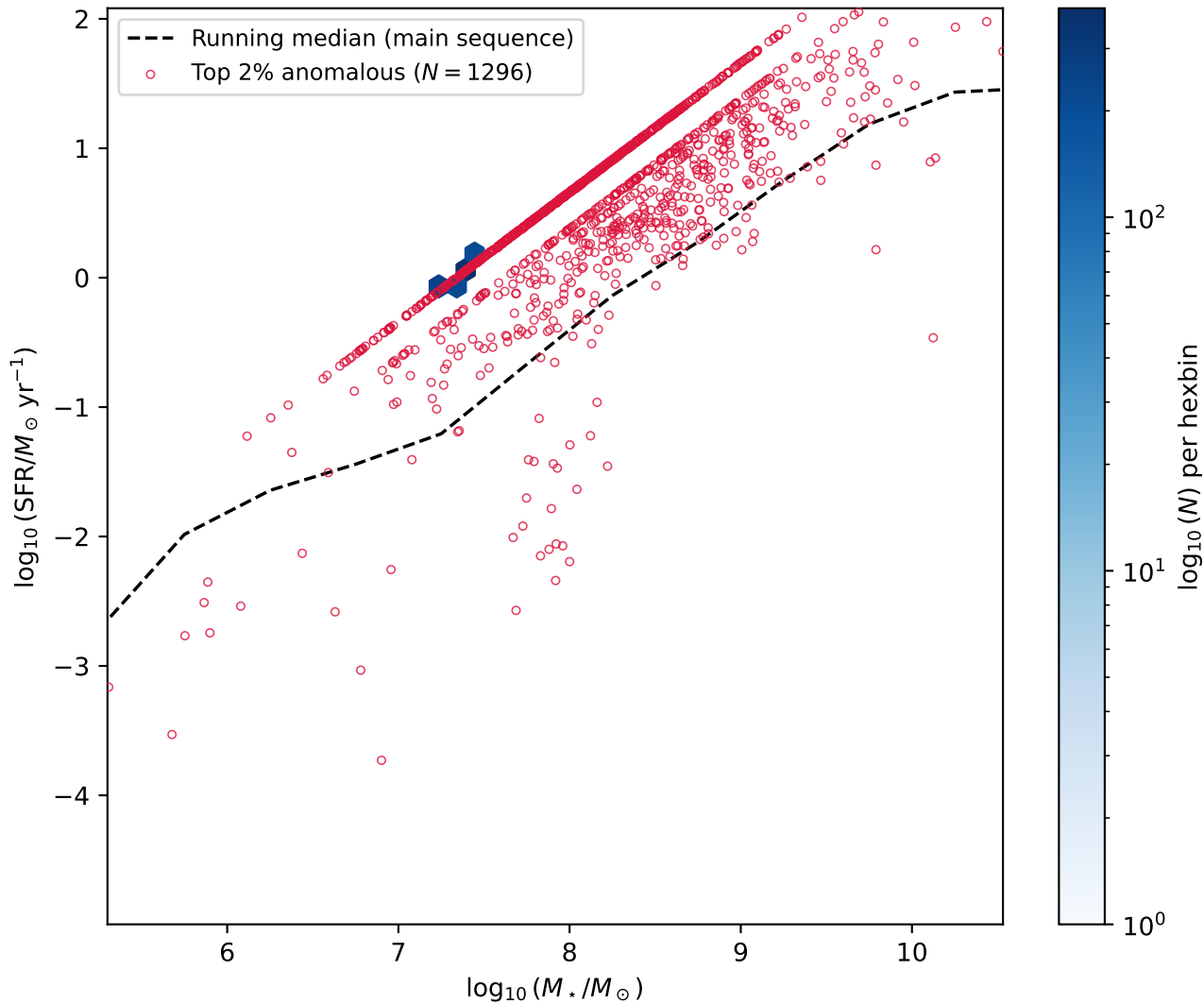
Anomalous sources across the stellar-mass-SFR plane
