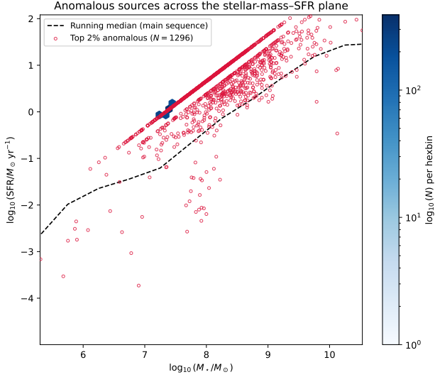
Figure 2. Top-2% flagged anomalies (crimson circles, N = 1,296 ) on the stellar-mass-SFR plane, against a hexbin density map of the full 64,195-source clean subsample with valid LePHARE mass/SFR fits. The dashed line is a running-median main-sequence trace (0.5 dex mass bins, \geq 10 sources/bin). Anomalies preferentially sit above this trace (Mann-Whitney U test on ensemble score, above vs. at/below the main sequence, p < 10^{-300} ).
