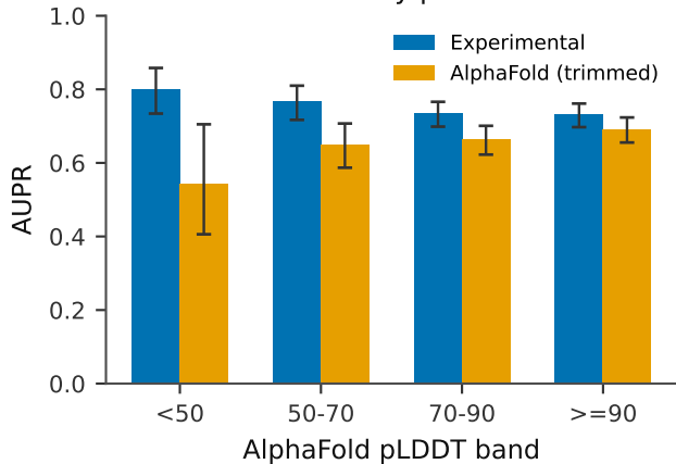
Pooled AUPR by pLDDT band
