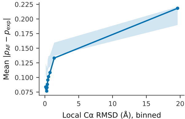
(a) Prediction shift vs. local RMSD
