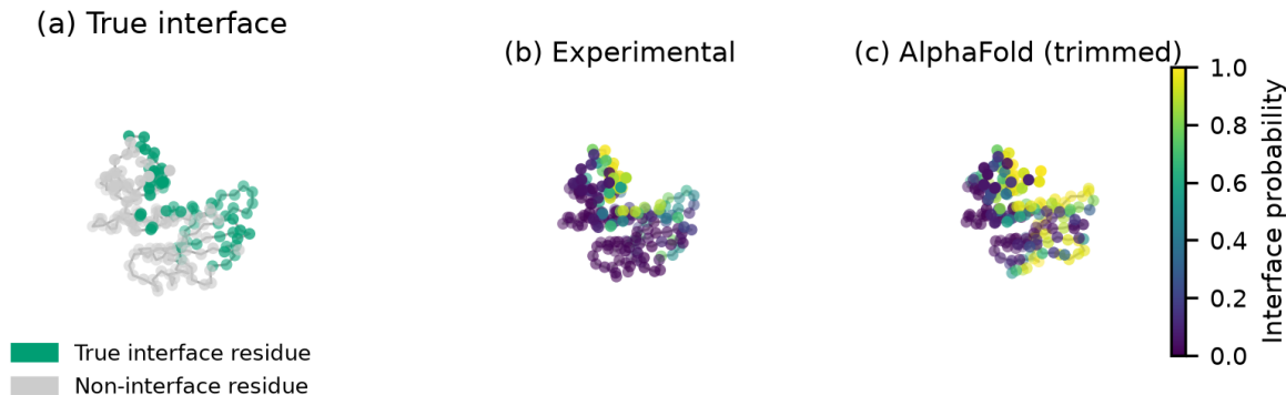
Figure 6: A representative chain (no headless 3D molecular renderer could be installed in this environment, so this is a matplotlib rendering of C \alpha positions colored by value, not a rendered surface – see Methods discussion in the accompanying repository documentation). (a) True interface residues (green) vs. non-interface (grey). (b) PeSTo’s per-residue interface probability from the experimental structure (AUPR 0.837 on this chain). (c) PeSTo’s per-residue interface probability from the AlphaFold model trimmed to the same residues (AUPR 0.806), superposed onto the experimental frame for comparison only (the underlying coordinates, and hence the prediction, come from the AlphaFold model).
